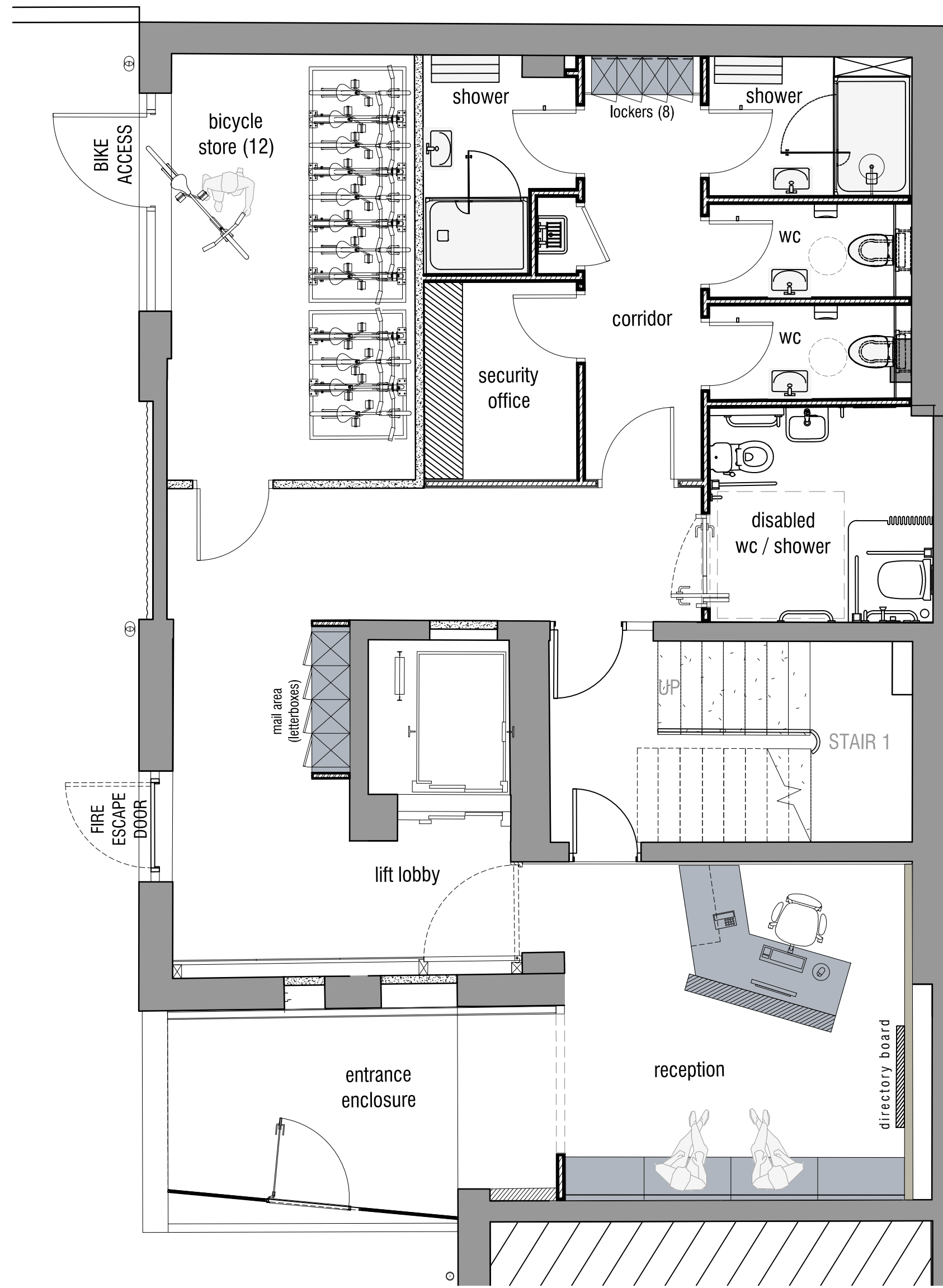
○ GROUND FLOOR SCALE 1:50
