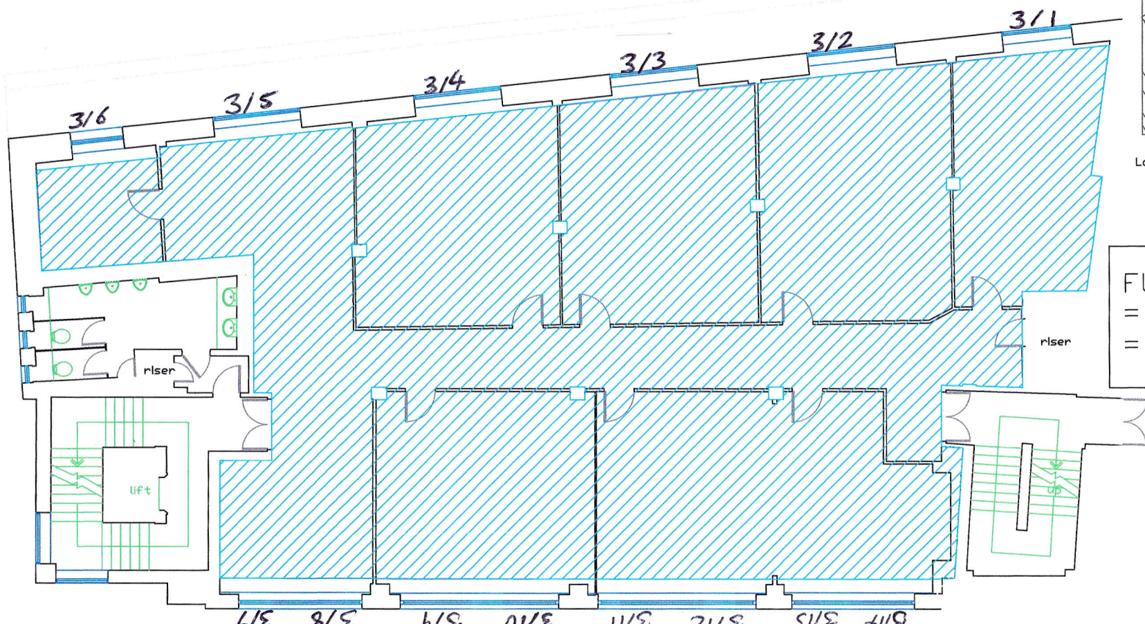
Third Floor 1:100
