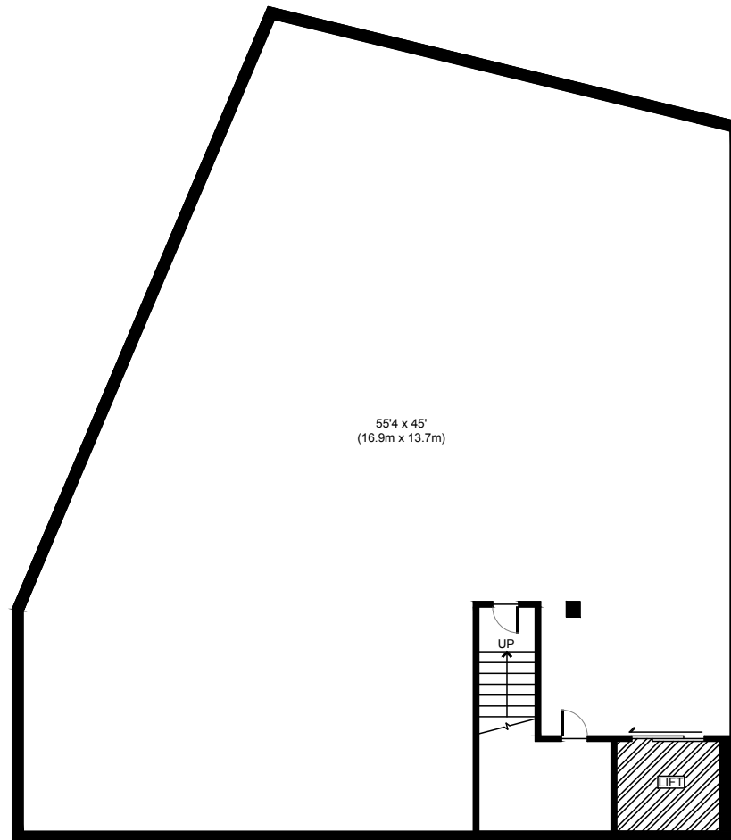
ANNEXE/BASEMENT AREA GROSS INTERNAL FLOOR AREA 2255 SQ FT
