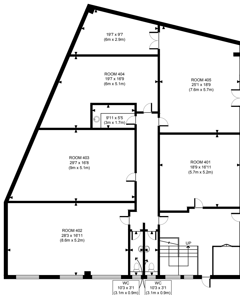
LOWER GROUND FLOOR GROSS INTERNAL FLOOR AREA 2803 SQ FT
