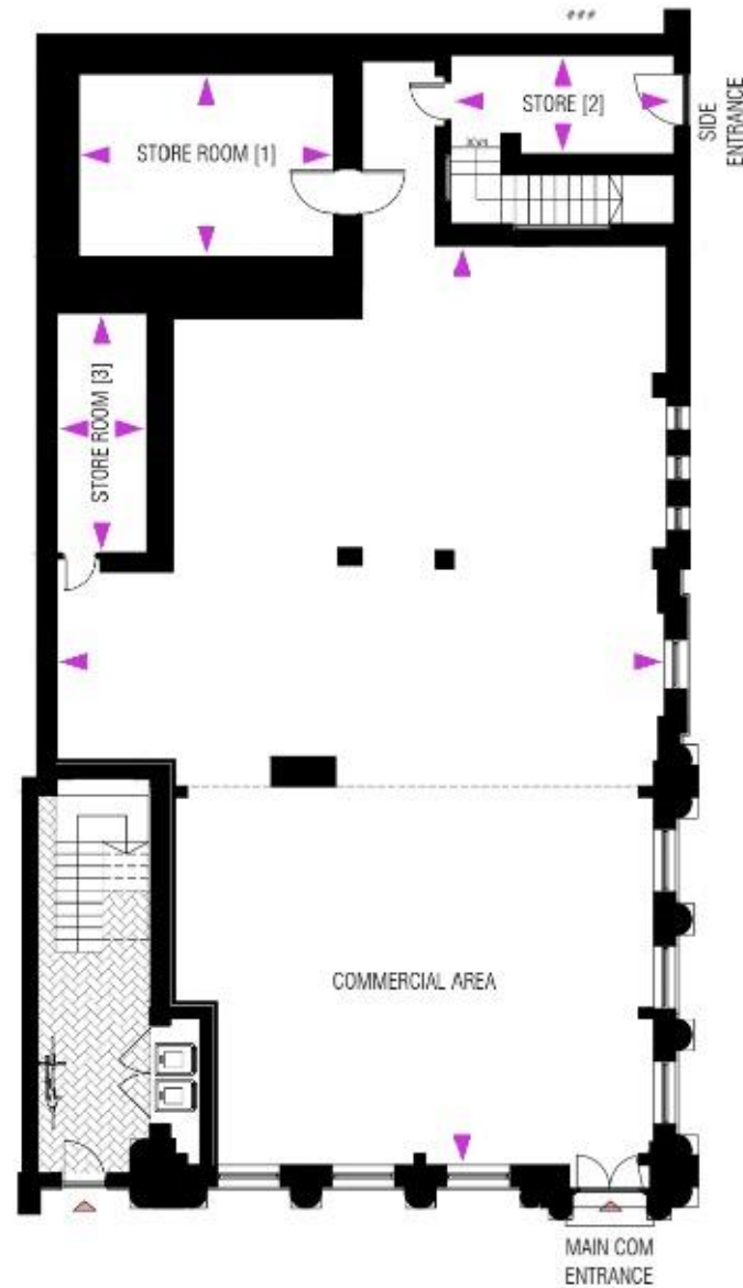
GROUND FLOOR PLAN SCALE: 1:100MM
