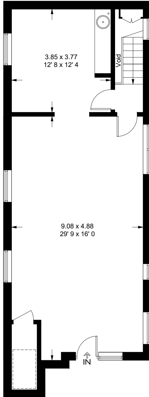
Ground Floor 682 sq ft / 63.3 sq m (Including Reduced Headroom / Excluding Void)
