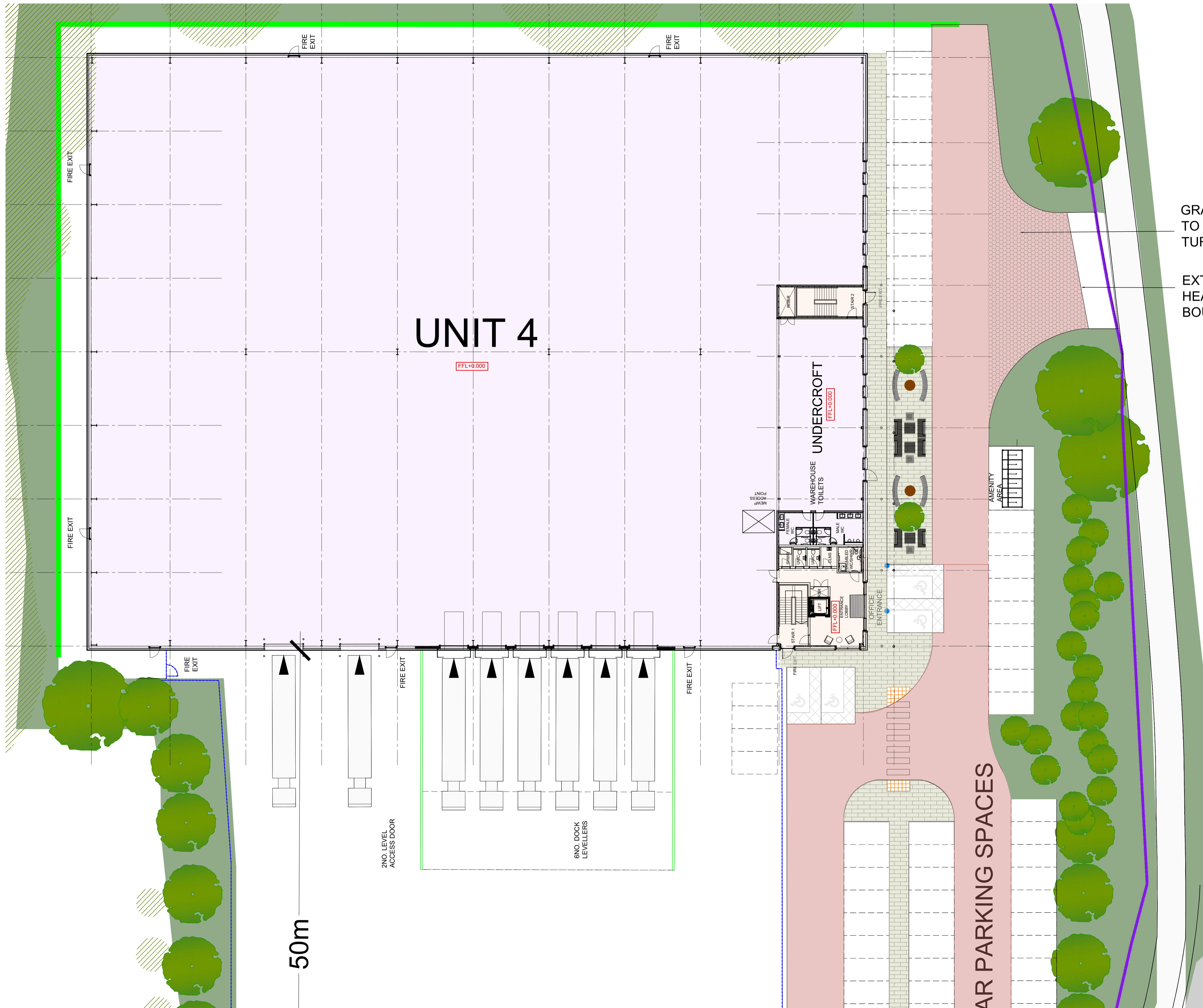
01 UNIT 4 - GROUND FLOOR PLAN 224 1:200
