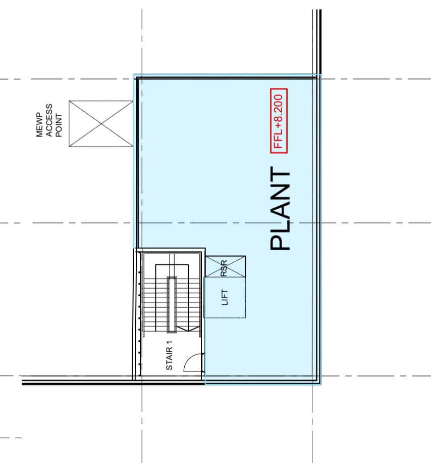
02 225 UNIT 4 - PLANT ROOM FLOOR PLAN 1:200
