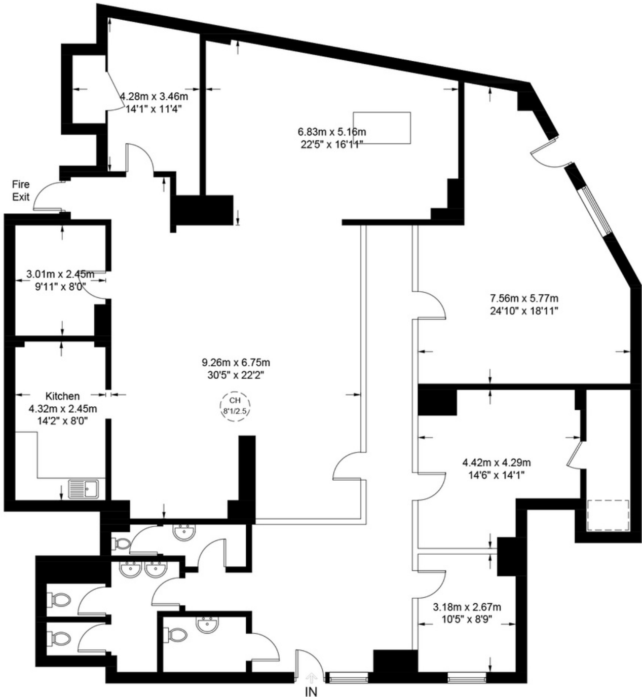
Ground Floor
